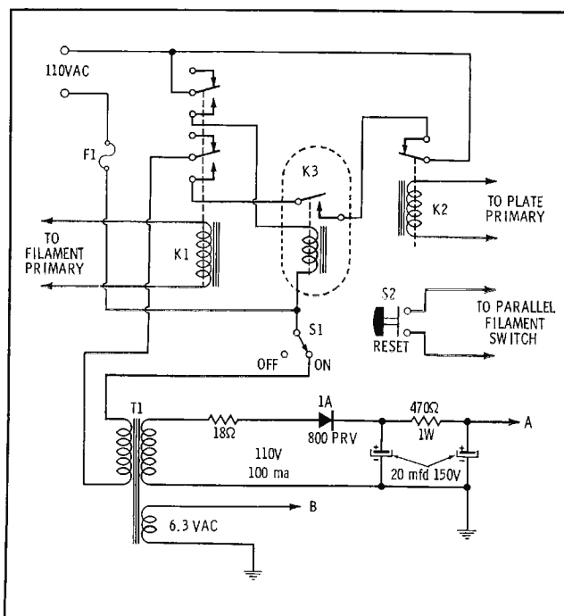
Fig. 2. Alarm control monitors power in transmitter plates.
