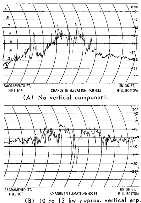
Fig. 6. Graphs of separation vs distance.
