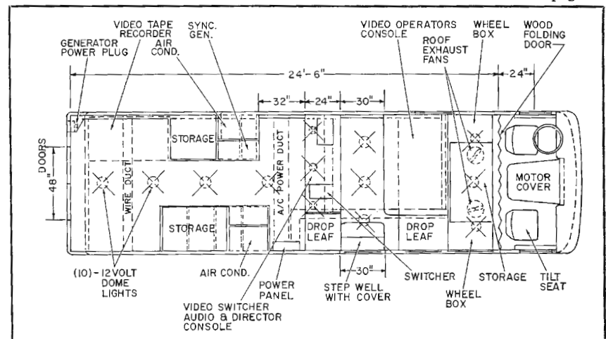
Fig. 4. Interior floor plan showing operating, storage, and equipment locations.
