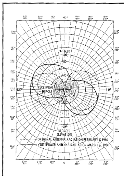
Fig. 3. Graph of radiation components.
