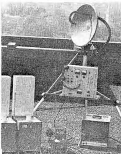
Fig. 3. Microwave link using TE power.
