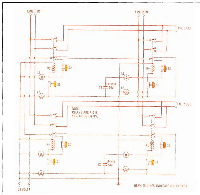
Fig. 2. Schematic diagram of a simple 2x2 electrical audio crossbar unit.
