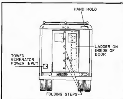
Fig. 6. Rear view showing access to roof.
