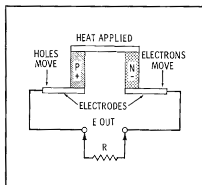
Fig. 1. Basic schematic of thermocouple.
