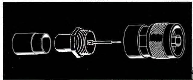
FULL CRIMP TYPE 75 OHM CONNECTOR
