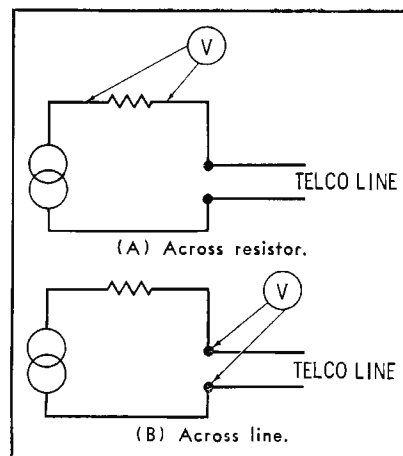
Fig. 3. VTVM positions in impedance test.
