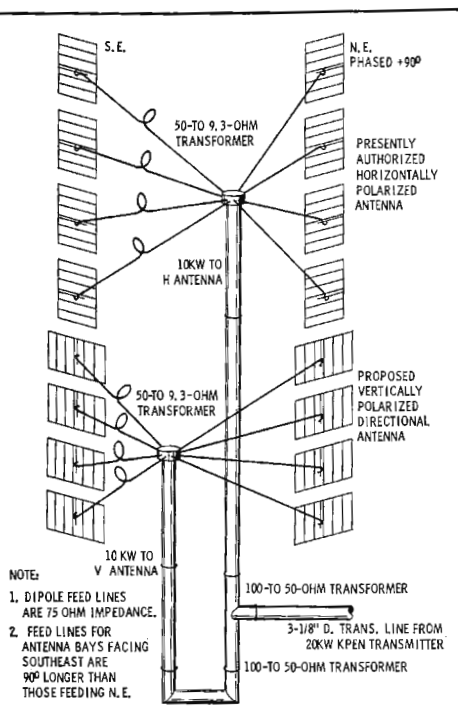
Fig. 1. Diagram of proposed antenna.
