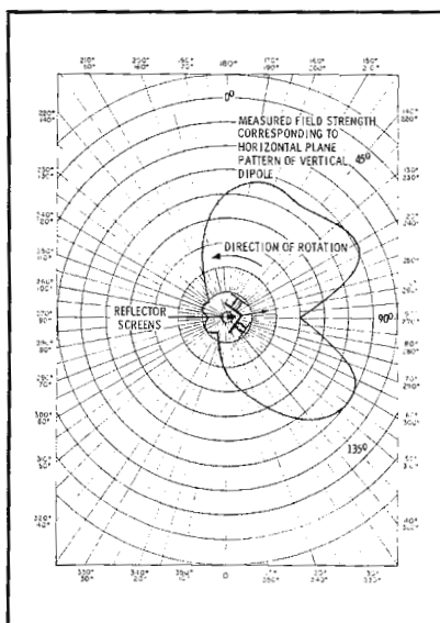
Fig. 2. A horizontal system field pattern.
