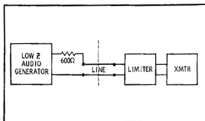
Fig. 1. Impedance measurements circuit.
